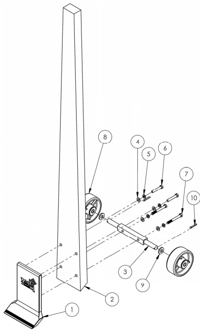
FIG. 1: PLB-series pry bars exploded parts diagram and bill of materials
